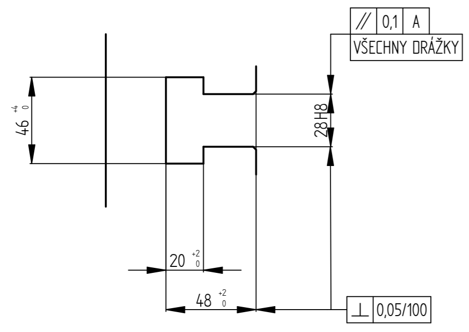
DETAIL B
